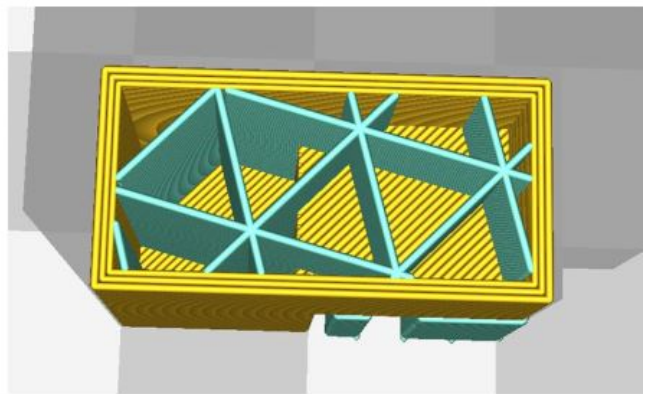
extruder_per_feature_infill
